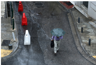
Heavy rain in Athens... 17_23093304
